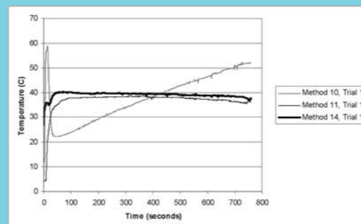
Figure 2: Temperature vs. time for trial 1 of method 10 (2 MREs on 500 mL), 11 (2 MRE on 500 mL for 10 minutes then remove fluid from heat source), and 14 (stove heating 500 mL to 75°C the remove from heat source). Time zero represents the beginning of the infusion. Delays of 6 min 15 sec, 11 min 5 sec, and 8 min 20 sec occurred prior to infusion for methods 10, 11, and 14 respectively. Note the spikes in the temperature of methods 10 at the beginning (58°C) and the end (52°C) of the infusion
